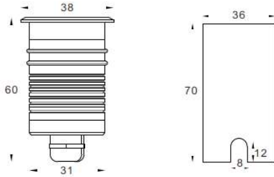
Physical Dimension(MM)
