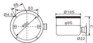
SS316L# Mounting sleeve
