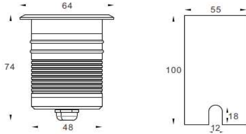
Physical Dimension(MM)
