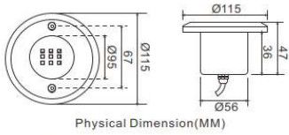
Physical Dimension(MM)
