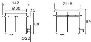
Mounting sleeve
