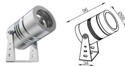
Underwater 1-3M
