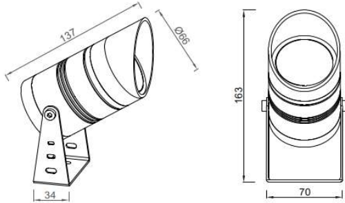
Physical Dimension(MM)
