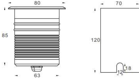
Physical Dimension(MM)
