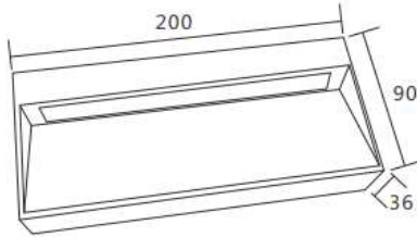
Physical Dimension(MM)
