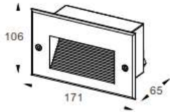
Physical Dimension(MM)
