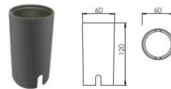
Mounting Sleeve(MM)
