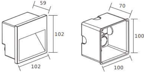
Physical Dimension(MM)
