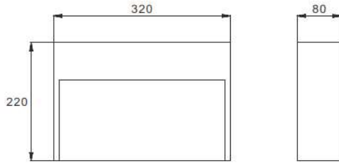
Physical Dimension(MM)
