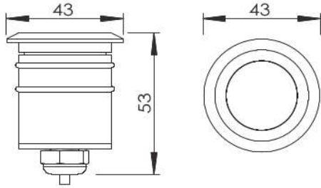
Physical Dimension(MM)
