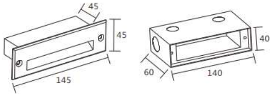
Physical Dimension(MM)
