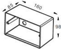
Mounting Sleeve(MM)
