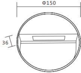
Physical Dimension(MM)
