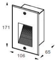
Physical Dimension(MM)
