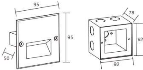
Physical Dimension(MM)
