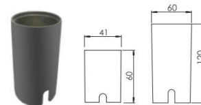
Mounting Sleeve(MM)
