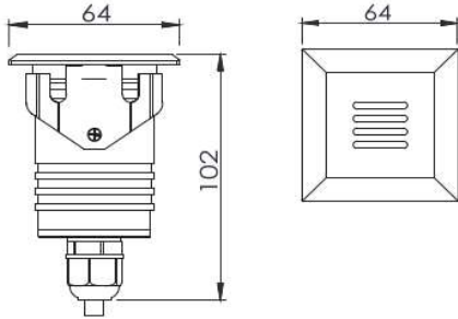
Physical Dimension(MM)
