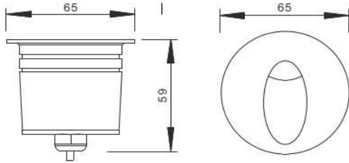
Physical Dimension(MM)
