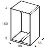
Mounting Sleeve(MM)
