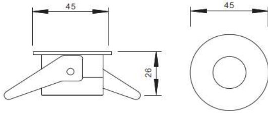
Physical Dimension(MM)
