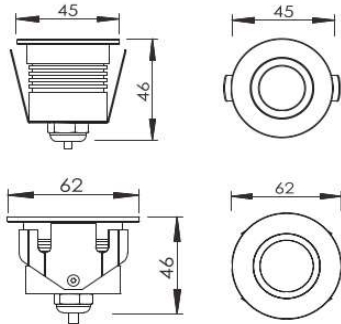
Physical Dimension(MM)
