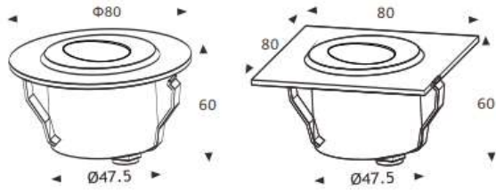
Physical Dimension(MM)
